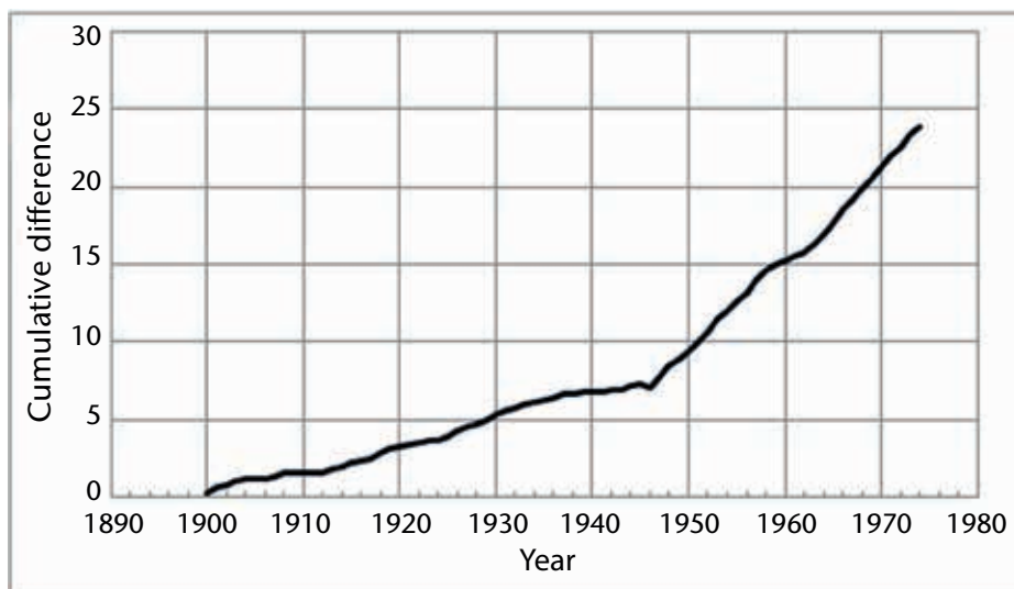
Figure 5.4. Example of a residual double-mass graph
